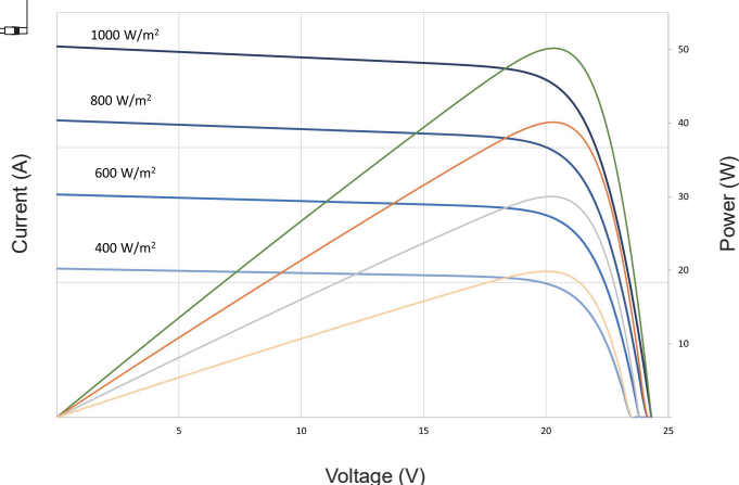
RNG-50DB-H Characteristics Versus Voltage
